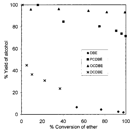
Figure 20. Effect of different substrates on the yield of alcohols. Substrate = 0.15 mol; \text{HNO}_3 = 4.77 M, 118 mL; \text{NaNO}_2 = 1 g; temperature = 90 °C; speed of stirring = 2500 rpm.
