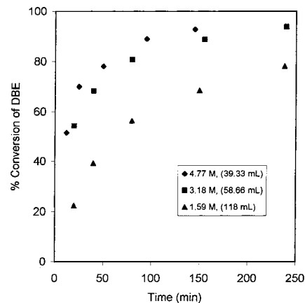
Figure 2. Effect of HNO 3 concentration on the conversion of DBE at constant mole ratio of the reactants. DBE = 0.15 mol; HNO 3 = 0.1875 mol; temperature = 90 °C; NaNO 2 = 1 g; speed of stirring = 2500 rpm.
