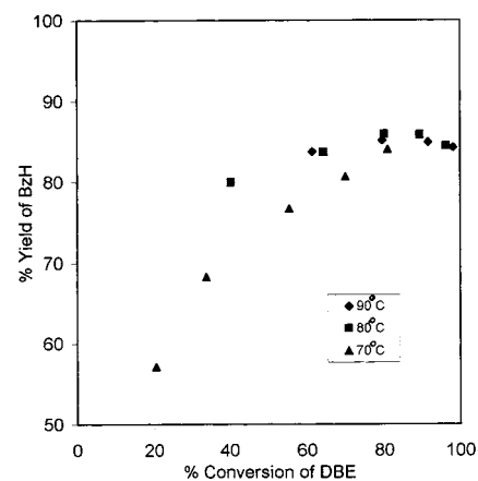
Figure 11. Effect of temperature on the yield of BzH. DBE = 0.15 mL; \text{HNO}_3 = 3.18 M, 79 mL; \text{NaNO}_2 = 1 g; speed of stirring = 2500 rpm.
