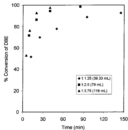
Figure 6. Effect of mole ratio of reactants on the conversion of DBE. DBE = 0.15 mol; HNO 3 = 4.77 M; NaNO 2 = 1 g; temperature = 90 °C; speed of stirring = 2500 rpm.
