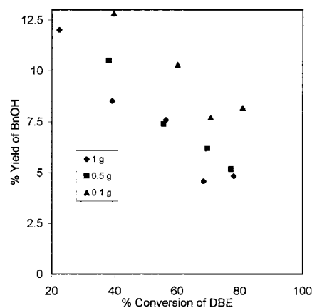
Figure 16. Effect of NaNO 2 loading on the yield of BnOH. DBE = 0.15 mol; HNO 3 = 1.59 M, 118 mL; temperature = 90 °C; speed of stirring = 2500 rpm.
