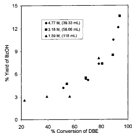
Figure 5. Effect of HNO 3 concentration on the yield of BzOH at constant mole ratio of the reactants. DBE = 0.15 mol; HNO 3 = 0.1875 mol; temperature = 90 °C; NaNO 2 = 1 g; speed of stirring = 2500 rpm.
