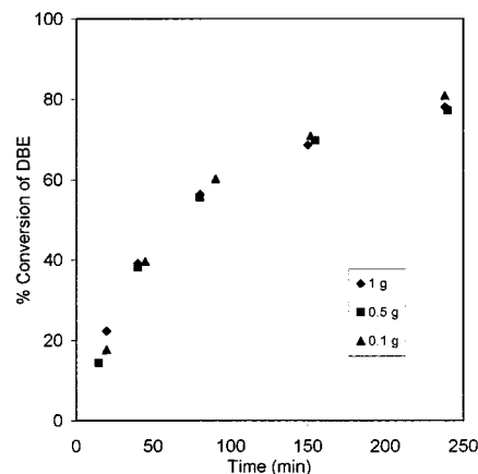
Figure 14. Effect of NaNO 2 loading on the conversion of DBE. DBE = 0.15 mol; HNO 3 = 1.59 M, 118 mL; temperature = 90 °C; speed of stirring = 2500 rpm.
