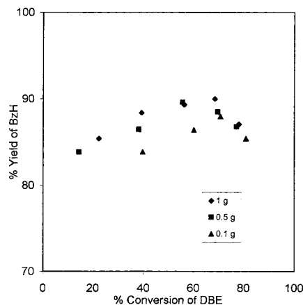
Figure 15. Effect of NaNO 2 loading on the yield of BzH. DBE = 0.15 mol; HNO 3 = 1.59 M, 118 mL; temperature = 90 °C; speed of stirring = 2500 rpm.
