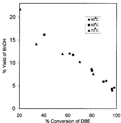
Figure 12. Effect of temperature on the yield of BnOH. DBE = 0.15 mL; HNO 3 = 3.18 M, 79 mL; NaNO 2 = 1 g; speed of stirring = 2500 rpm.
