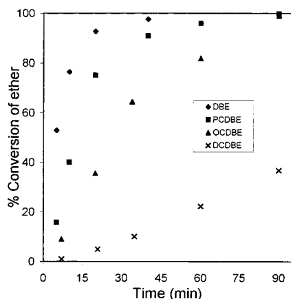
Figure 18. Effect of different substrates on the conversion. Substrate = 0.15 mol; \text{HNO}_3 = 4.77 M, 118 mL; \text{NaNO}_2 = 1 g; temperature = 90 °C; speed of stirring = 2500 rpm.
