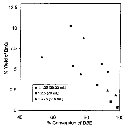
Figure 8. Effect of mole ratio of reactants on the yield of BnOH. DBE = 0.15 mol; \text{HNO}_3 = 4.77 M; \text{NaNO}_2 = 1 g; temperature = 90 °C; speed of stirring = 2500 rpm.
