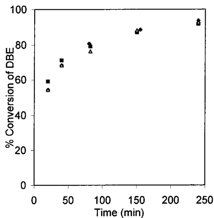
Figure 1. Effect of speed of stirring on the progress of reaction at 90 °C. ◆: DBE = 0.15 mol; HNO 3 = 3.18 M, 59 mL; NaNO 2 = 1 g; speed of stirring = 2500 rpm. ■: DBE = 0.15 mol; HNO 3 = 3.18 M, 59 mL; NaNO 2 = 1 g; speed of stirring = 1500 rpm. □: DBE = 1.05 mol; HNO 3 = 3.18 M, 413 mL; NaNO 2 = 7 g; speed of stirring = 1500 rpm.
