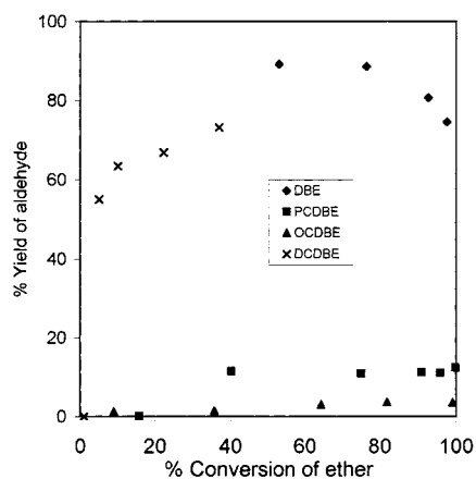
Figure 19. Effect of different substrates on the yield of aldehyde. Substrate = 0.15 mol; \text{HNO}_3 = 4.77 M, 118 mL; \text{NaNO}_2 = 1 g; temperature = 90 °C; speed of stirring = 2500 rpm.
