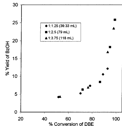
Figure 9. Effect of mole ratio of reactants on the yield of BzOH. DBE = 0.15 mol; \text{HNO}_3 = 4.77 M; \text{NaNO}_2 = 1 g; temperature = 90 °C; speed of stirring = 2500 rpm.
