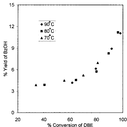
Figure 13. Effect of temperature on the yield of BzOH. DBE = 0.15 mL; HNO 3 = 3.18 M, 79 mL; NaNO 2 = 1 g; speed of stirring = 2500 rpm.
