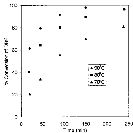
Figure 10. Effect of temperature on the conversion of DBE. DBE = 0.15 mL; \text{HNO}_3 = 3.18 M, 79 mL; \text{NaNO}_2 = 1 g; speed of stirring = 2500 rpm.
