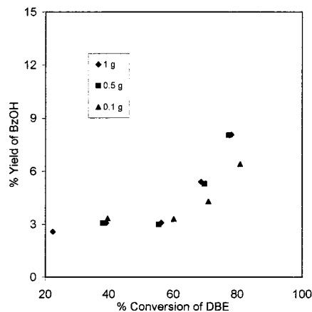
Figure 17. Effect of \text{NaNO}_2 loading on the yield of BzOH. DBE = 0.15 mol; \text{HNO}_3 = 1.59 M, 118 mL; temperature = 90 °C; speed of stirring = 2500 rpm.
