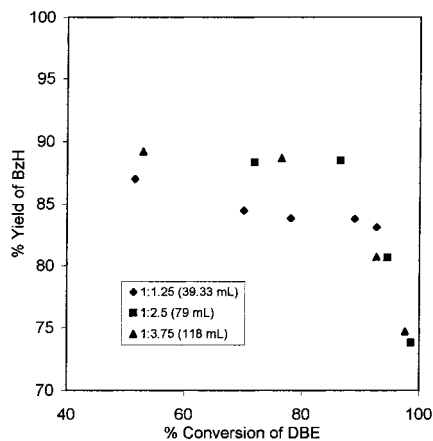
Figure 7. Effect of mole ratio of reactants on the yield of BzH. DBE = 0.15 mol; \text{HNO}_3 = 4.77 M; \text{NaNO}_2 = 1 g; temperature = 90 °C; speed of stirring = 2500 rpm.
