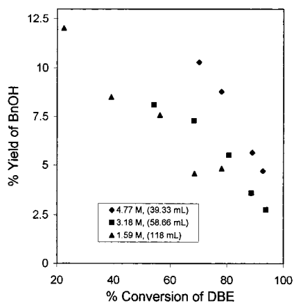
Figure 4. Effect of HNO 3 concentration on the yield of BnOH at constant mole ratio of the reactants. DBE = 0.15 mol; HNO 3 = 0.1875 mol; temperature = 90 °C; NaNO 2 = 1 g; speed of stirring = 2500 rpm.
