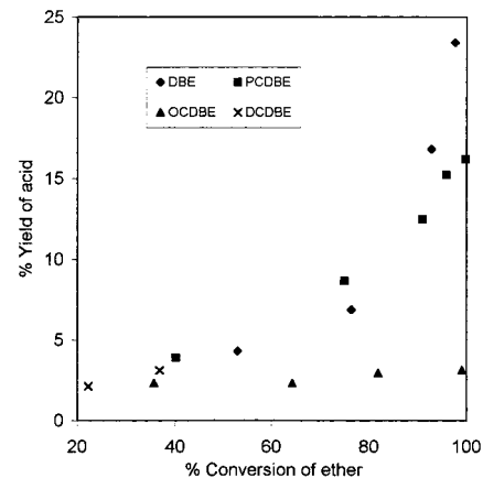
Figure 21. Effect of different substrates on the yield of acid. Substrate = 0.15 mol; \text{HNO}_3 = 4.77 M, 118 mL; \text{NaNO}_2 = 1 g; temperature = 90 °C; speed of stirring = 2500 rpm.
