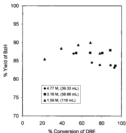
Figure 3. Effect of HNO 3 concentration on the yield of BzH at constant mole ratio of the reactants. DBE = 0.15 mol; HNO 3 = 0.1875 mol; temperature = 90 °C; NaNO 2 = 1 g; speed of stirring = 2500 rpm.
